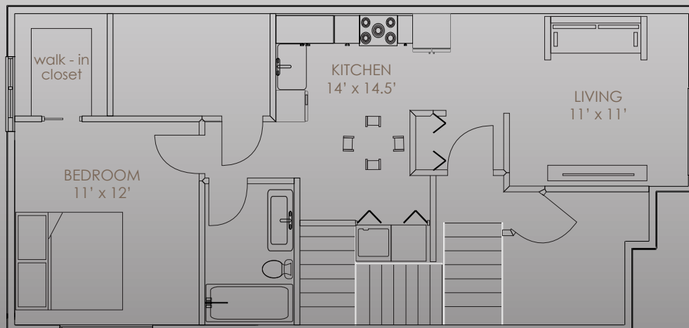
PROPOSED BASEMENT
